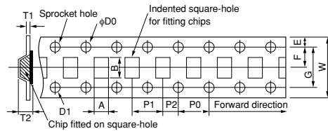
Tape Dimensions
